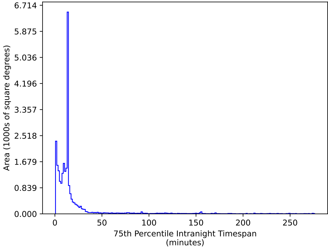
too_elab_heavy_r128_d2_gz_v3.4_10yrs All sky i band: 75th Percentile Intranight Timespan
