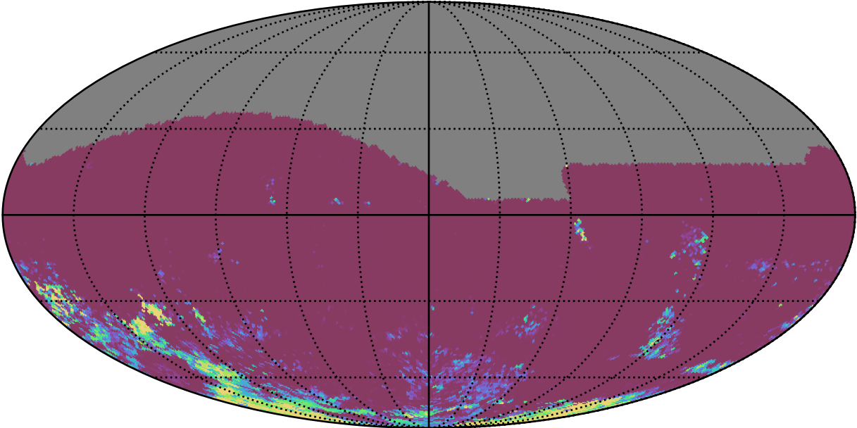
too_elab_heavy_r128_d2_gz_v3.4_10yrs All sky gr bands: 75th Percentile Intranight Timespan
