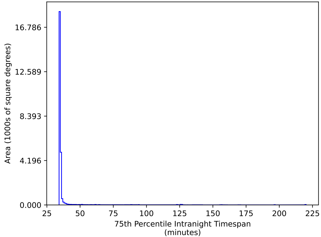
too_elab_heavy_r128_d2_gz_v3.4_10yrs All sky gr bands: 75th Percentile Intranight Timespan
