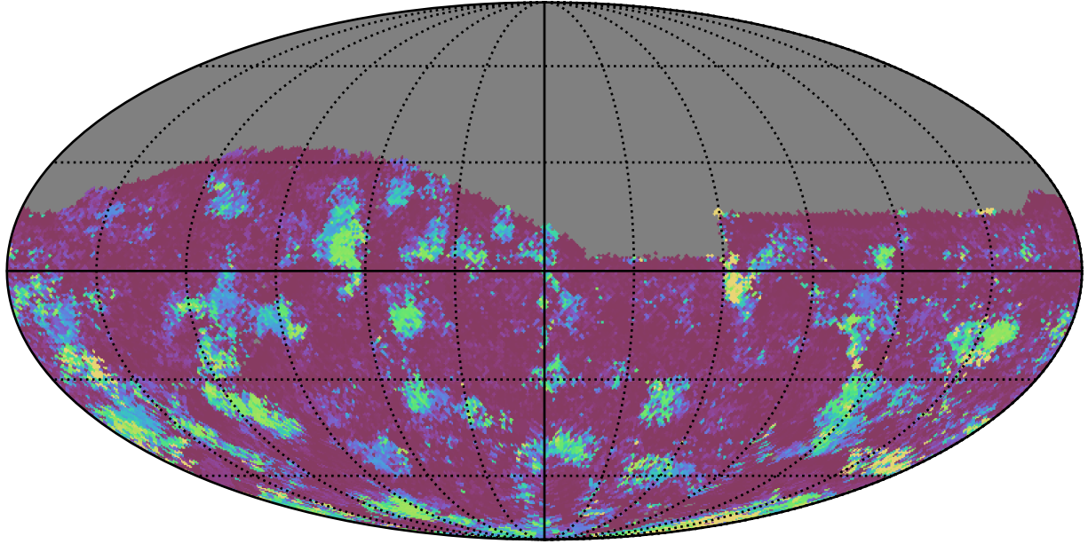
too_elab_heavy_r128_d2_gz_v3.4_10yrs All sky g band: 75th Percentile Intranight Timespan
