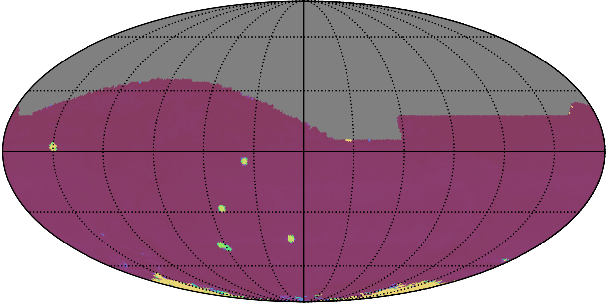
too_elab_heavy_r128_d2_gz_v3.4_10yrs All sky all bands: 75th Percentile Intranight Timespan
