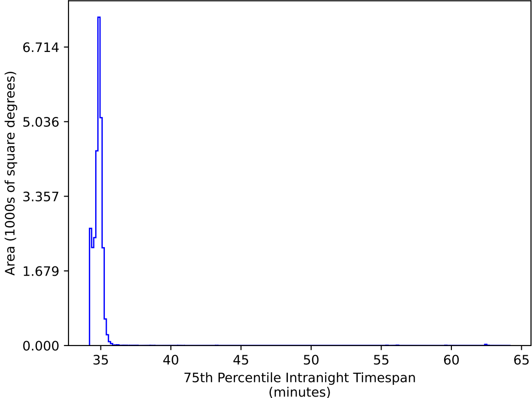
too_elab_heavy_r128_d2_gz_v3.4_10yrs All sky: 75th Percentile Intranight Timespan
