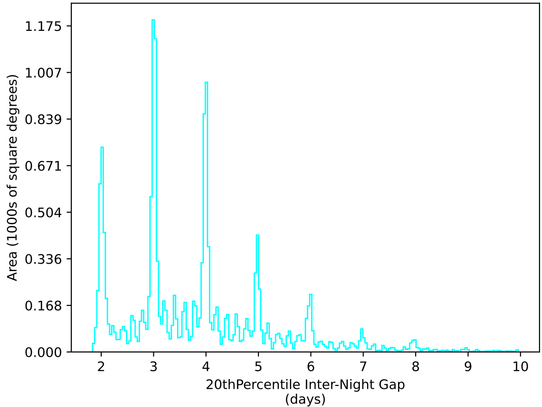
too_elab_heavy_r128_d2_gz_v3.4_10yrs WFD u band: 20thPercentile Inter-Night Gap
