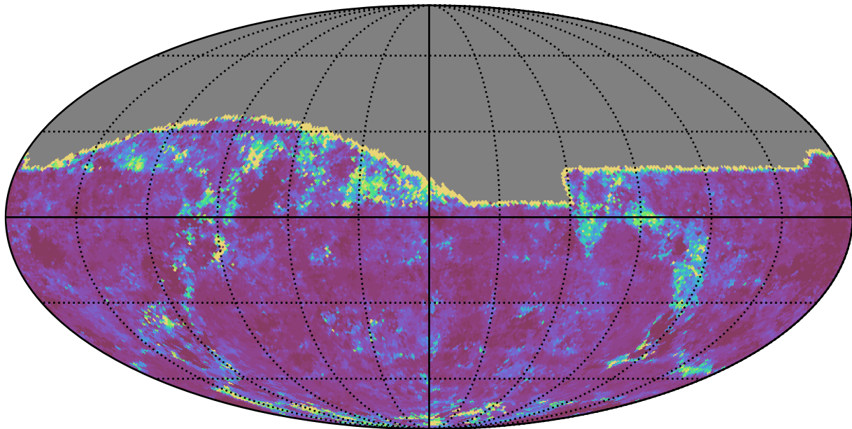
too_elab_heavy_r128_d2_gz_v3.4_10yrs All sky g band: 20thPercentile Inter-Night Gap
