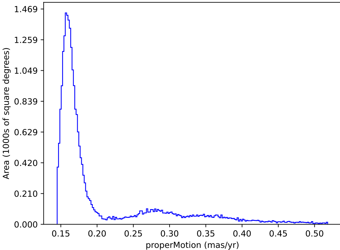
too_elab_heavy_r128_d2_gz_v3.4_10yrs : properMotion
