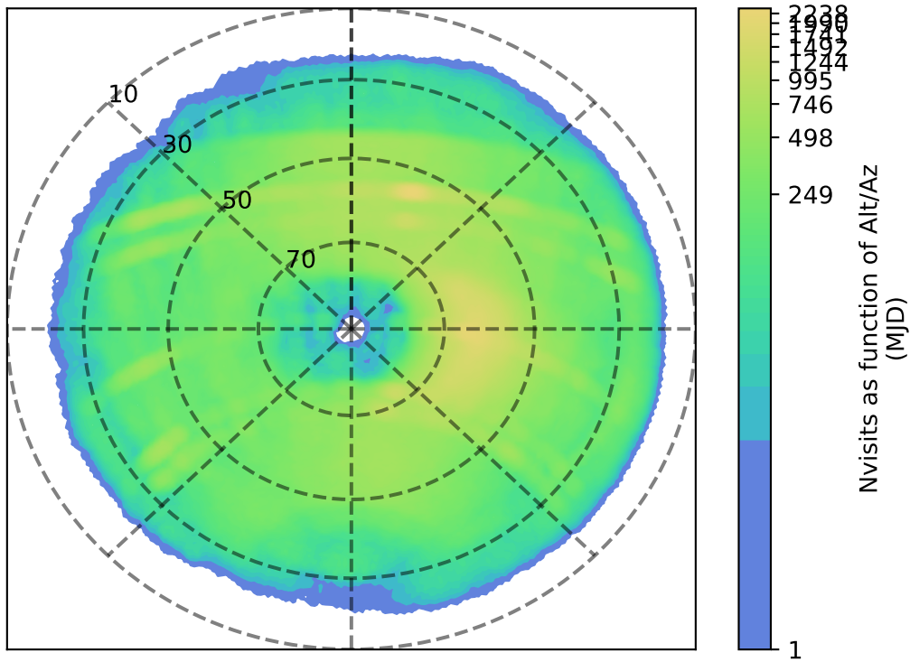
too_elab_heavy_r128_d2_gz_v3.4_10yrs z: Nvisits as function of Alt/Az
