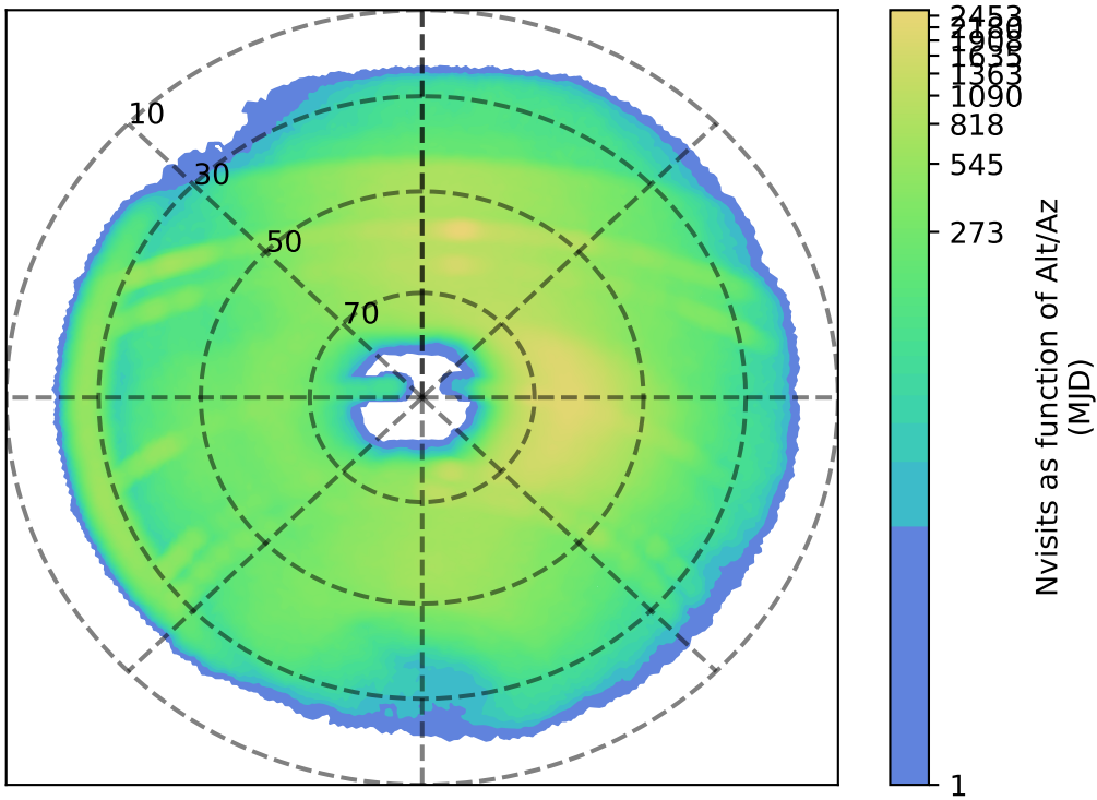
too_elab_heavy_r128_d2_gz_v3.4_10yrs r: Nvisits as function of Alt/Az
