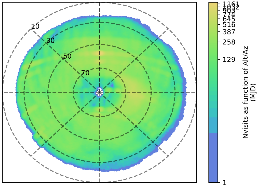
too_elab_heavy_r128_d2_gz_v3.4_10yrs g: Nvisits as function of Alt/Az
