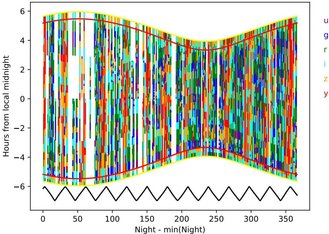
too_elab_heavy_r128_d2_gz_v3.4_10yrs year 9-10: Hourglass
