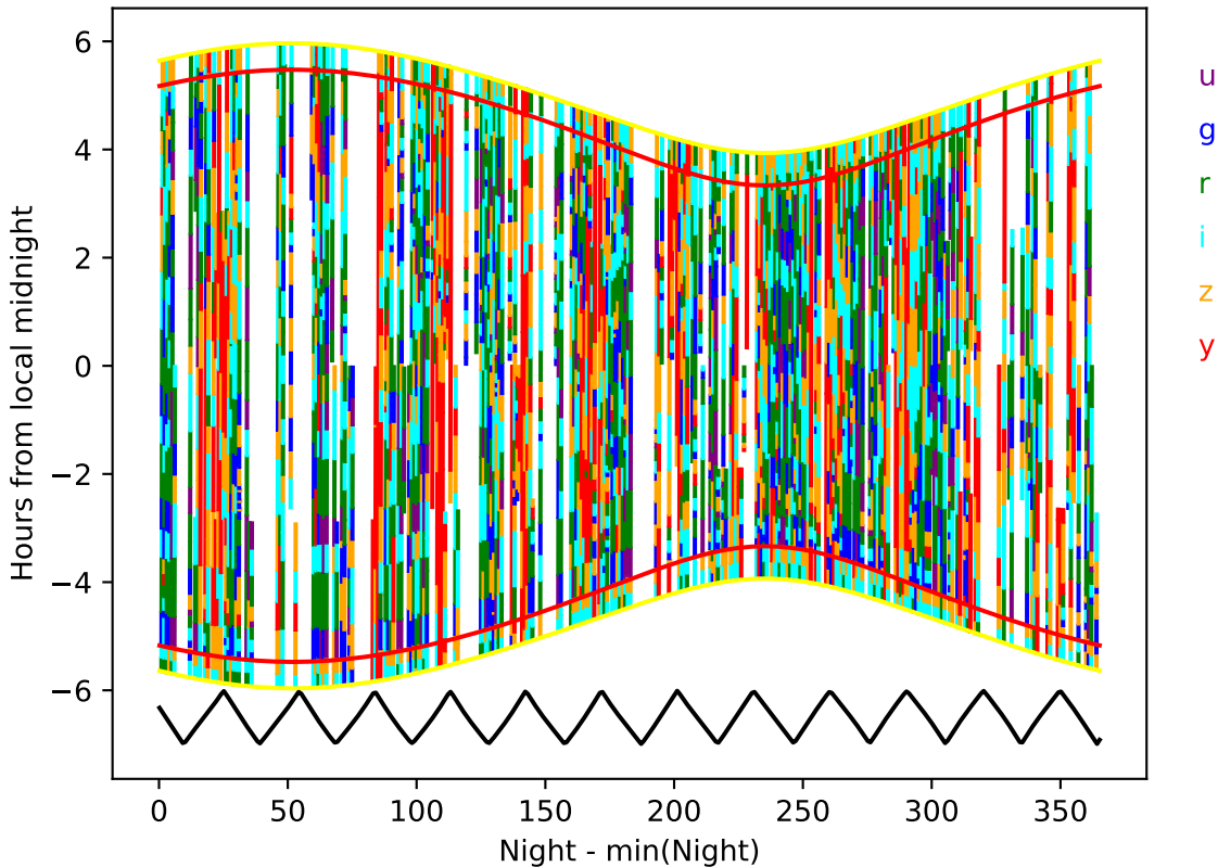
too_elab_heavy_r128_d2_gz_v3.4_10yrs year 7-8: Hourglass
