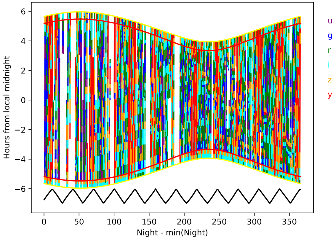
too_elab_heavy_r128_d2_gz_v3.4_10yrs year 0-1: Hourglass
