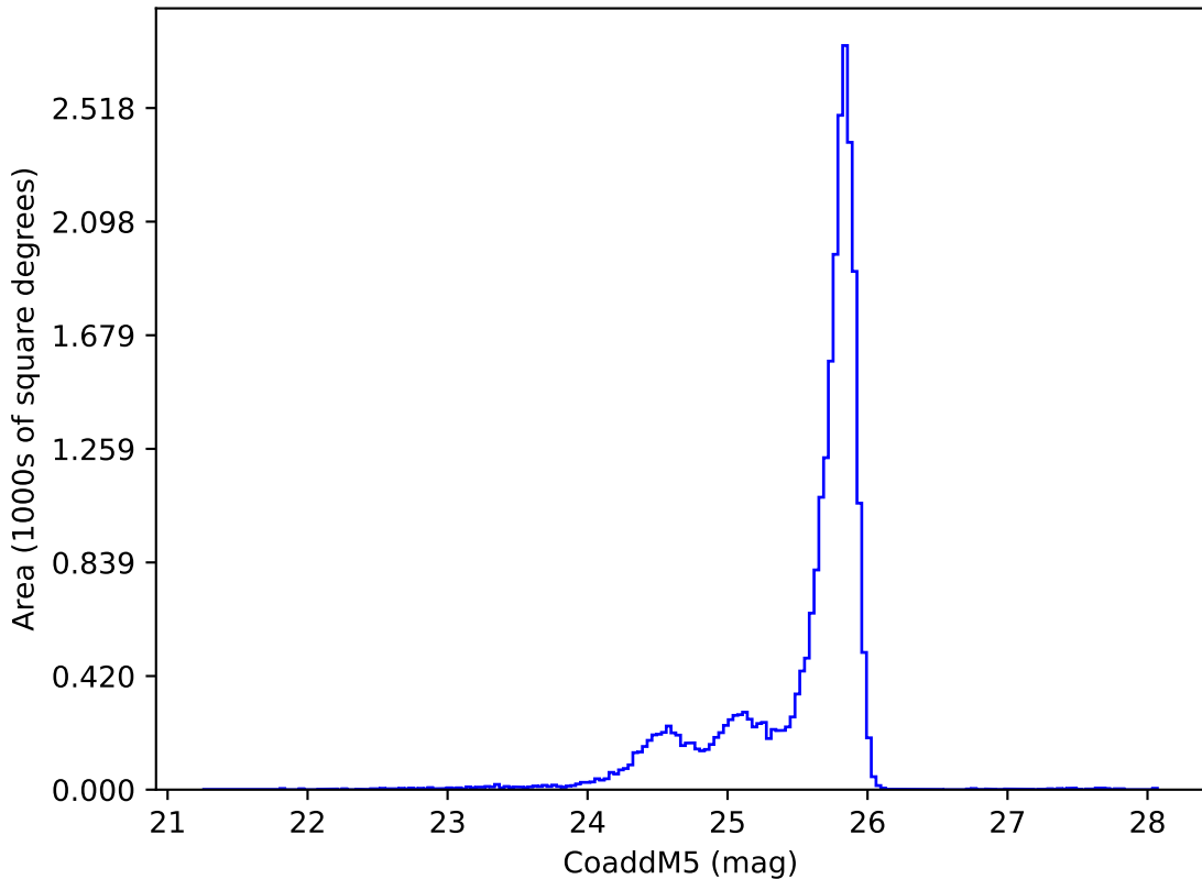
too_elab_heavy_r128_d2_gz_v3.4_10yrs z: CoaddM5
