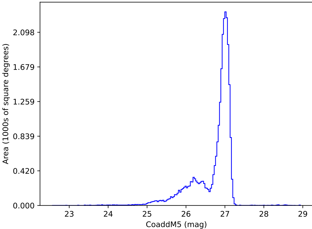
too_elab_heavy_r128_d2_gz_v3.4_10yrs r: CoaddM5
