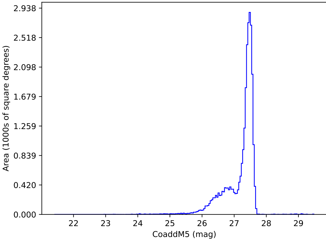
too_elab_heavy_r128_d2_gz_v3.4_10yrs : CoaddM5
