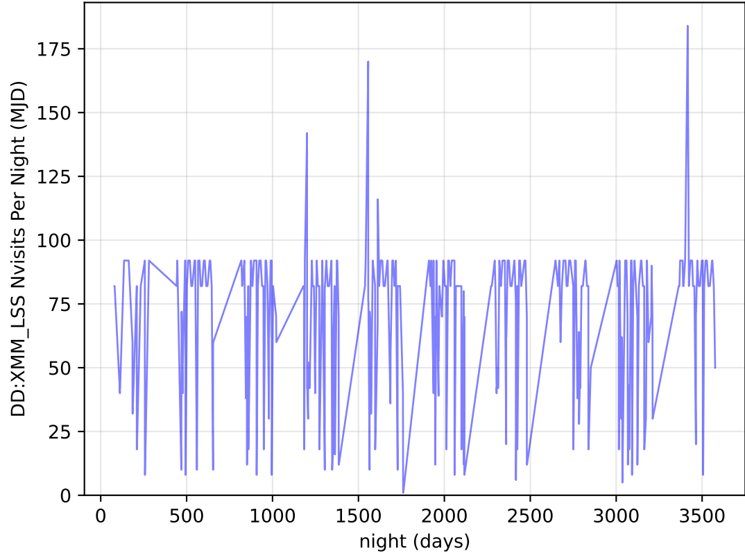
too_elab_heavy_r128_d2_gz_v3.4_10yrs all bands: DD:XMM_LSS Nvisits Per Night
