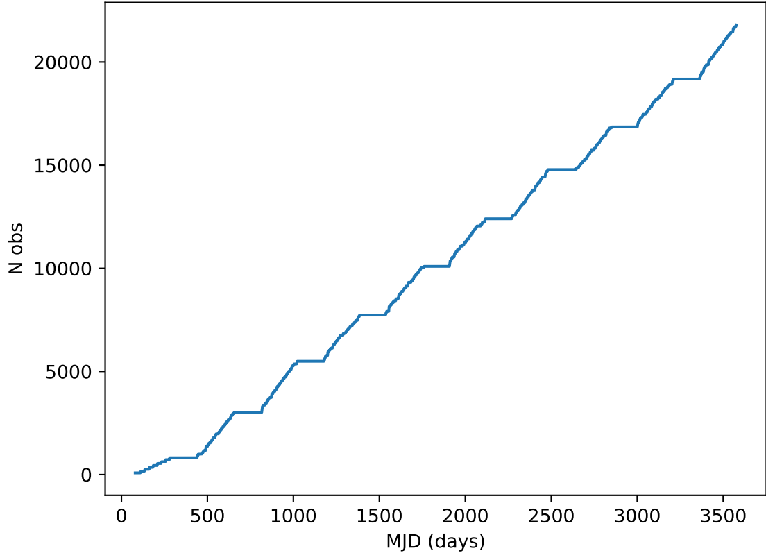
too_elab_heavy_r128_d2_gz_v3.4_10yrs all bands: DD:XMM_LSS Cumulative NVisits
