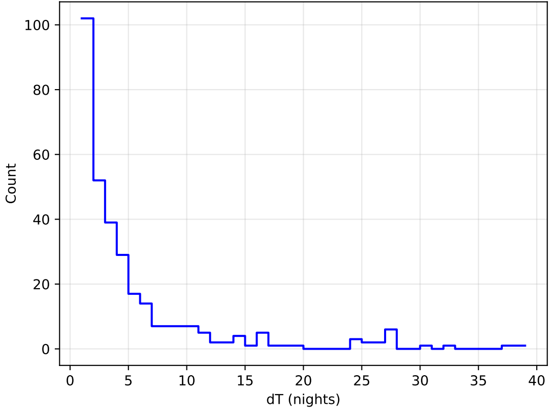
too_elab_heavy_r128_d2_gz_v3.4_10yrs all bands: DD:WFD Delta Nights Histogram
