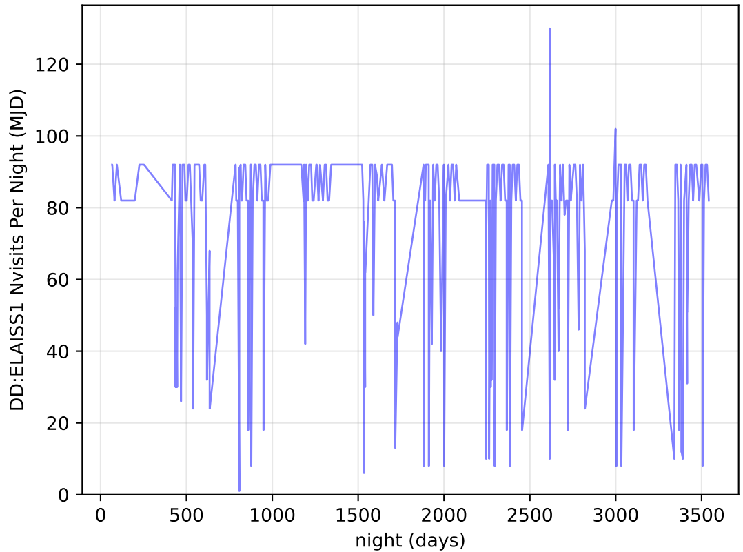
too_elab_heavy_r128_d2_gz_v3.4_10yrs all bands: DD:ELAISS1 Nvisits Per Night
