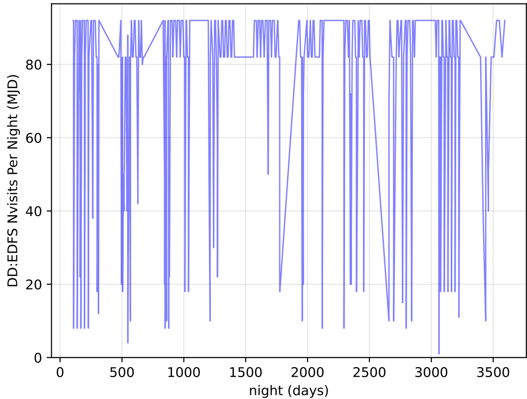
too_elab_heavy_r128_d2_gz_v3.4_10yrs all bands: DD:EDFS Nvisits Per Night
