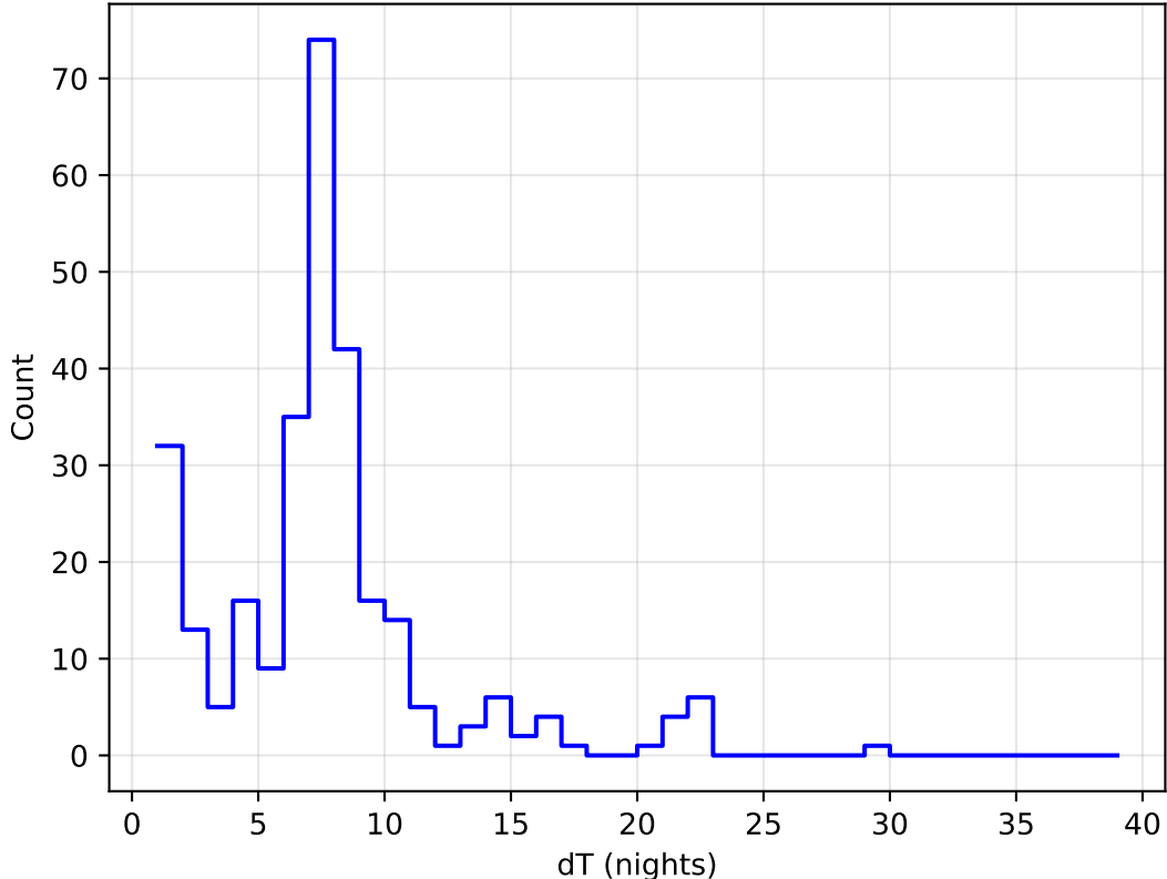
too_elab_heavy_r128_d2_gz_v3.4_10yrs all bands: DD:EDFS Delta Nights Histogram
