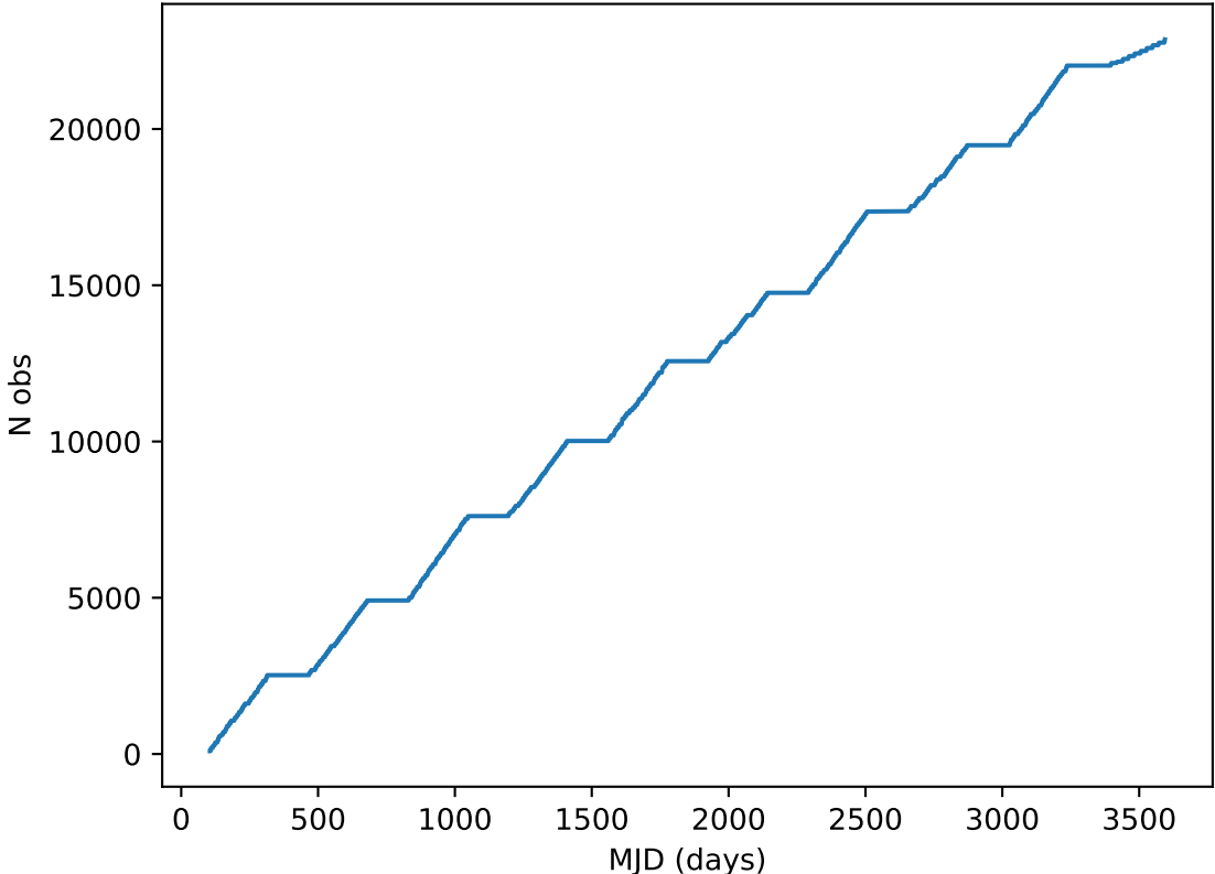
too_elab_heavy_r128_d2_gz_v3.4_10yrs all bands: DD:EDFS Cumulative NVisits
