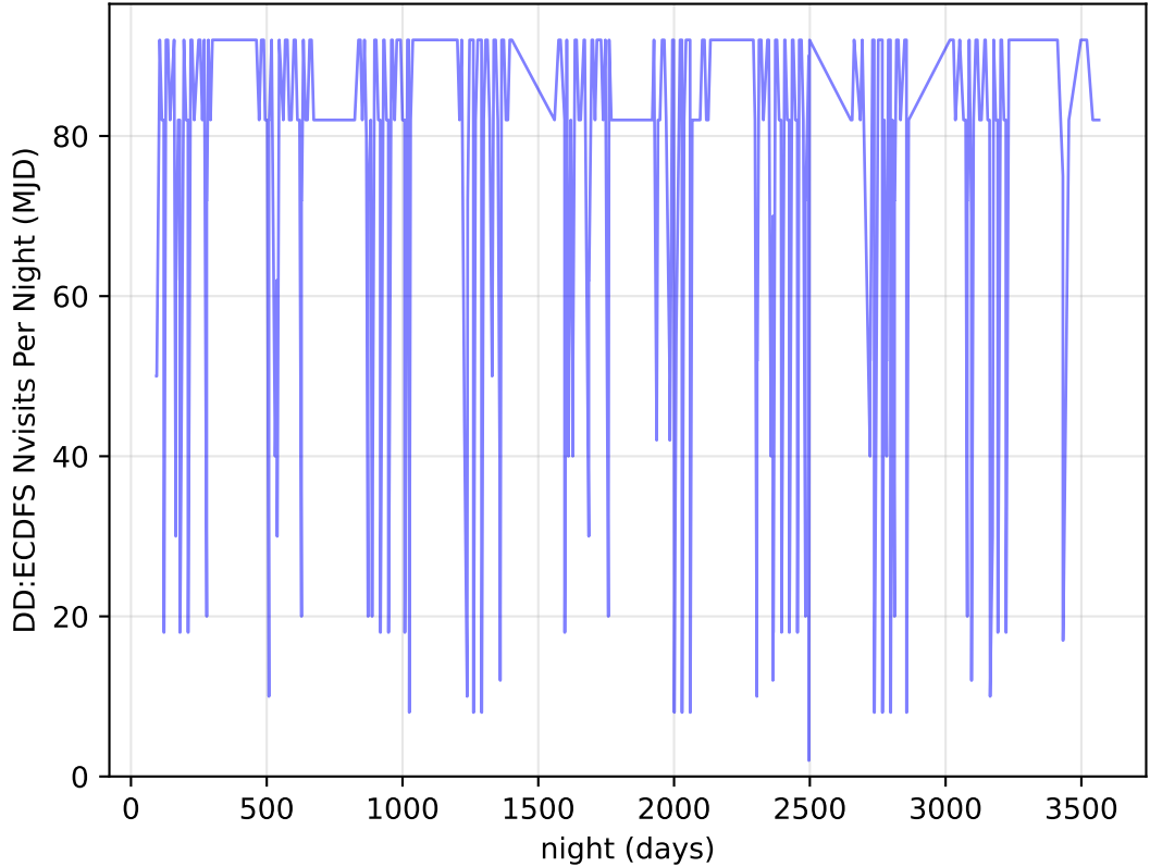
too_elab_heavy_r128_d2_gz_v3.4_10yrs all bands: DD:ECDFS Nvisits Per Night
