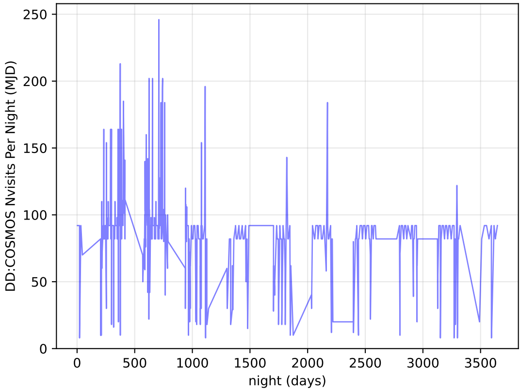
too_elab_heavy_r128_d2_gz_v3.4_10yrs all bands: DD: COSMOS Nvisits Per Night
