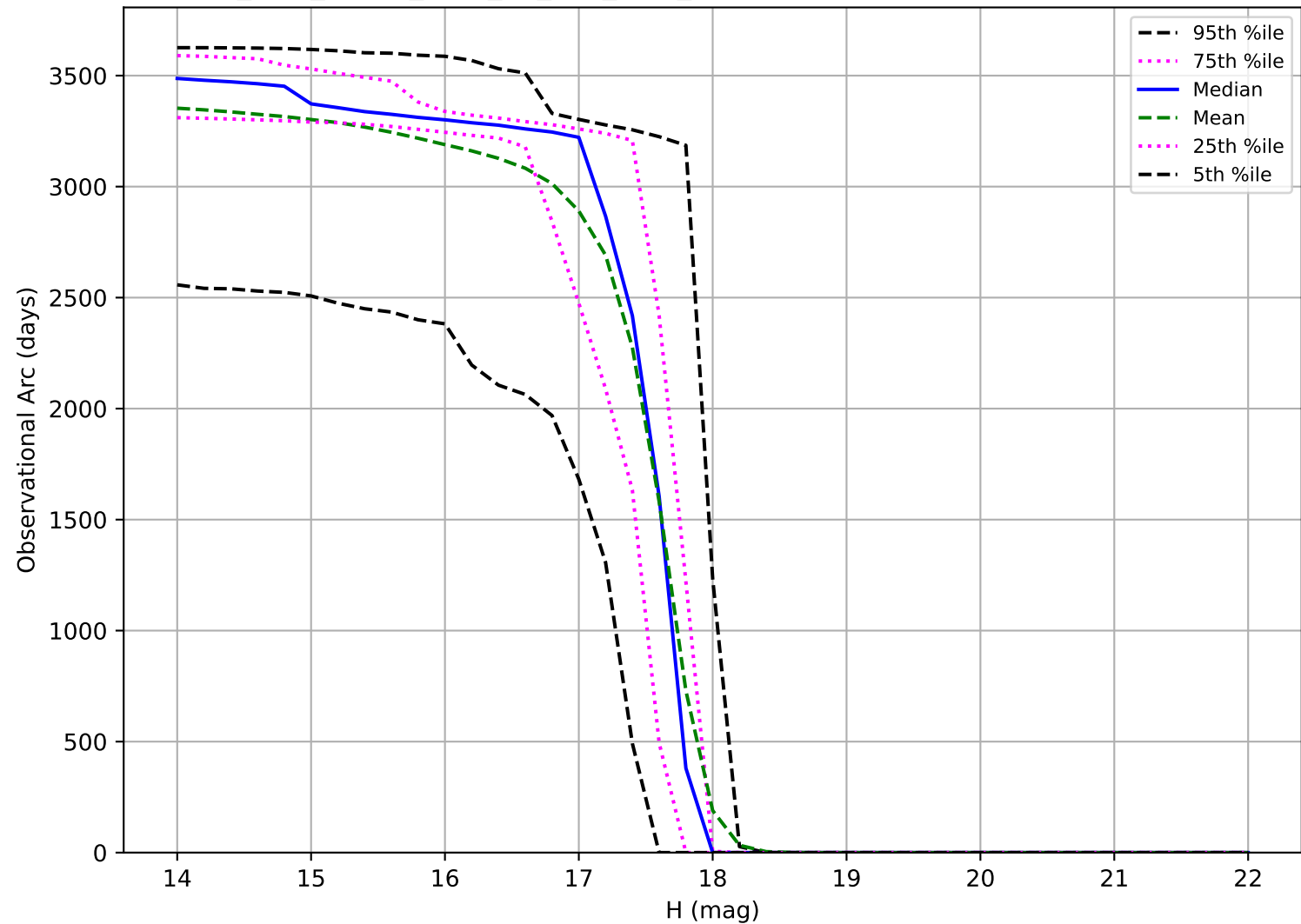
too_elab_heavy_r128_d2_griz_v3.4_10yrs: Observational Arc Length Trojan
