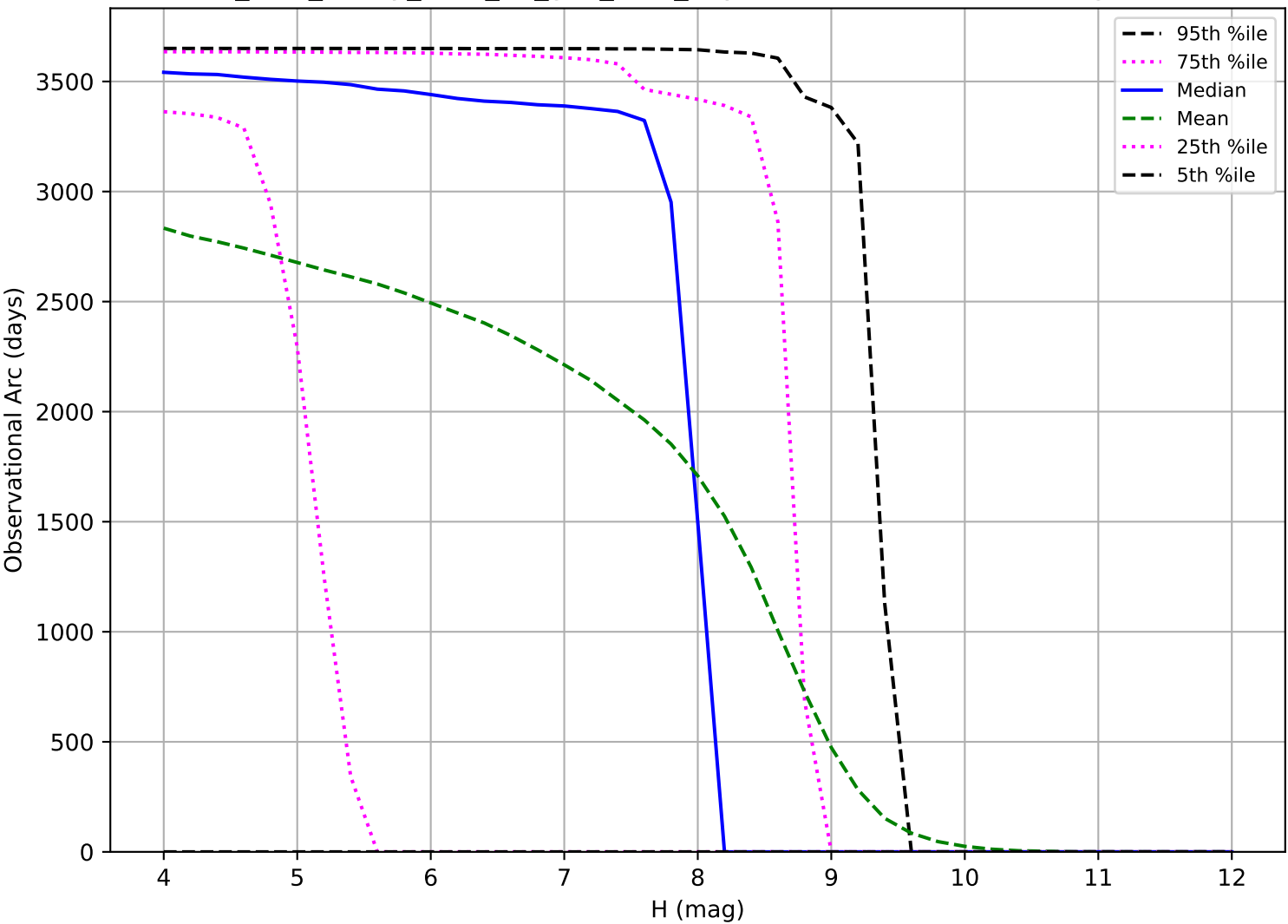
too_elab_heavy_r128_d2_griz_v3.4_10yrs: Observational Arc Length TNO
