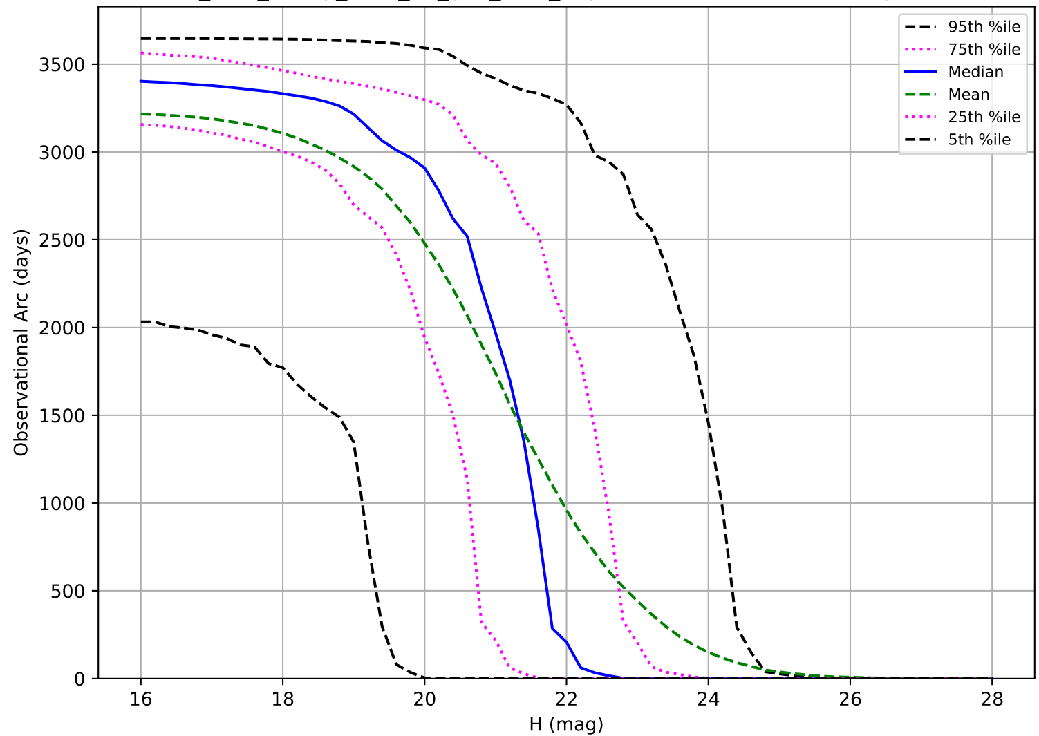
too_elab_heavy_r128_d2_griz_v3.4_10yrs: Observational Arc Length PHA
