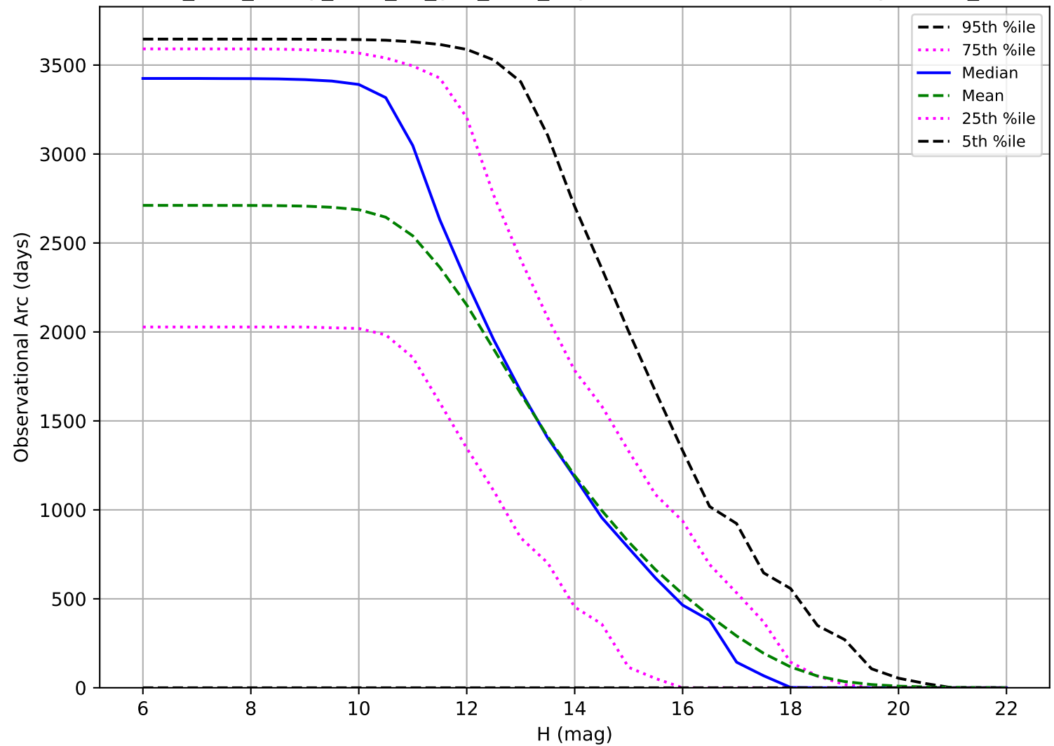
too_elab_heavy_r128_d2_griz_v3.4_10yrs: Observational Arc Length OCC_r5
