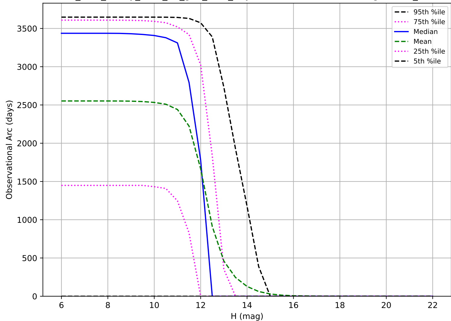
too_elab_heavy_r128_d2_griz_v3.4_10yrs: Observational Arc Length OCC_r20
