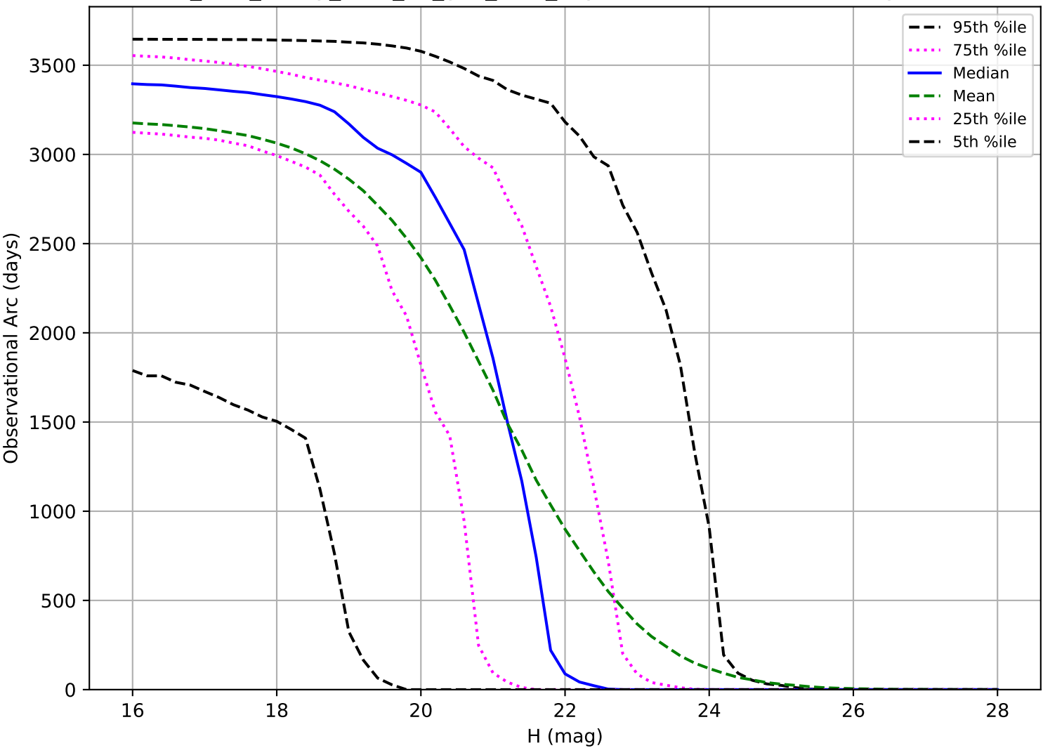
too_elab_heavy_r128_d2_griz_v3.4_10yrs: Observational Arc Length NEO
