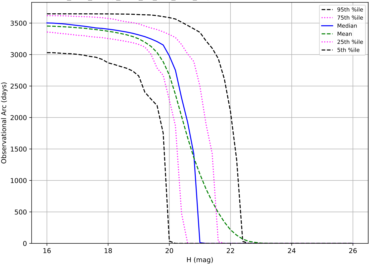
too_elab_heavy_r128_d2_griz_v3.4_10yrs: Observational Arc Length MBA
