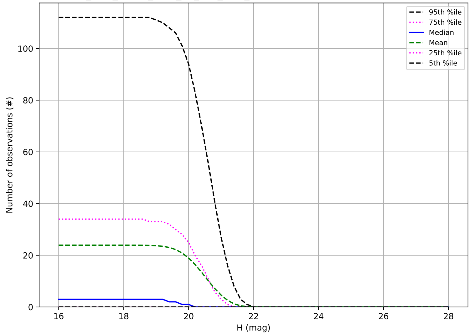
too_elab_heavy_r128_d2_griz_v3.4_10yrs: Number of observations Vatira
