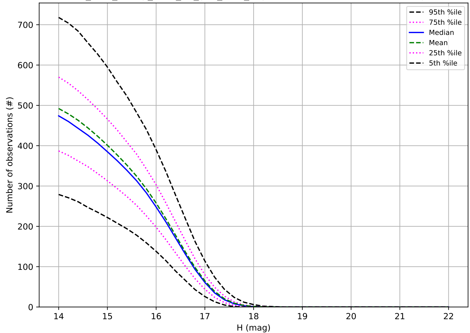
too_elab_heavy_r128_d2_griz_v3.4_10yrs: Number of observations Trojan
