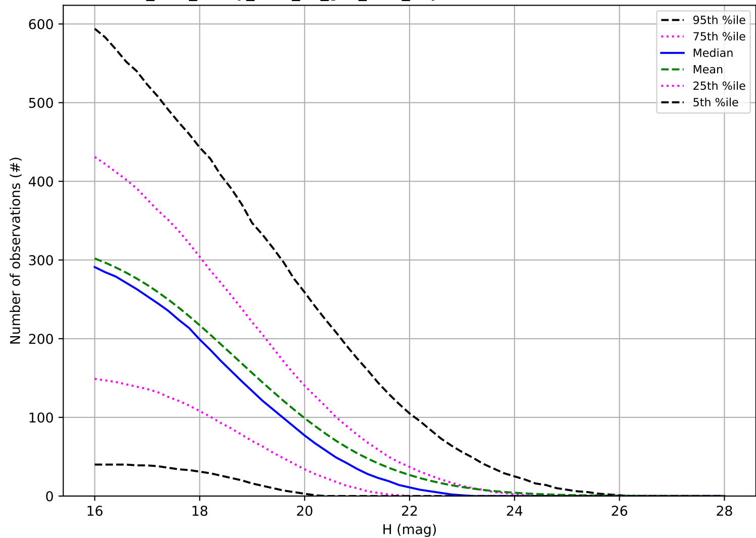
too_elab_heavy_r128_d2_griz_v3.4_10yrs: Number of observations PHA
