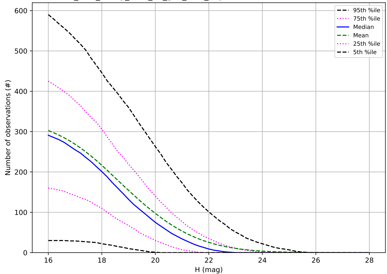
too_elab_heavy_r128_d2_griz_v3.4_10yrs: Number of observations NEO
