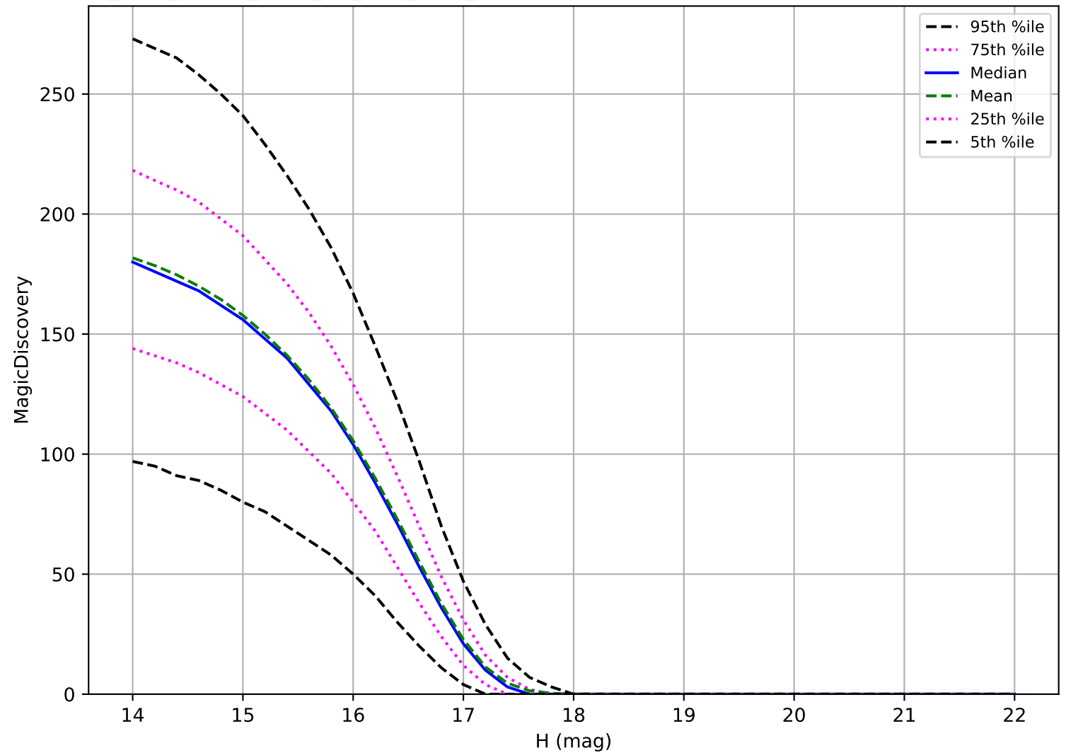
too_elab_heavy_r128_d2_griz_v3.4_10yrs: Trojan 6 detections in 60 nights detection loss
