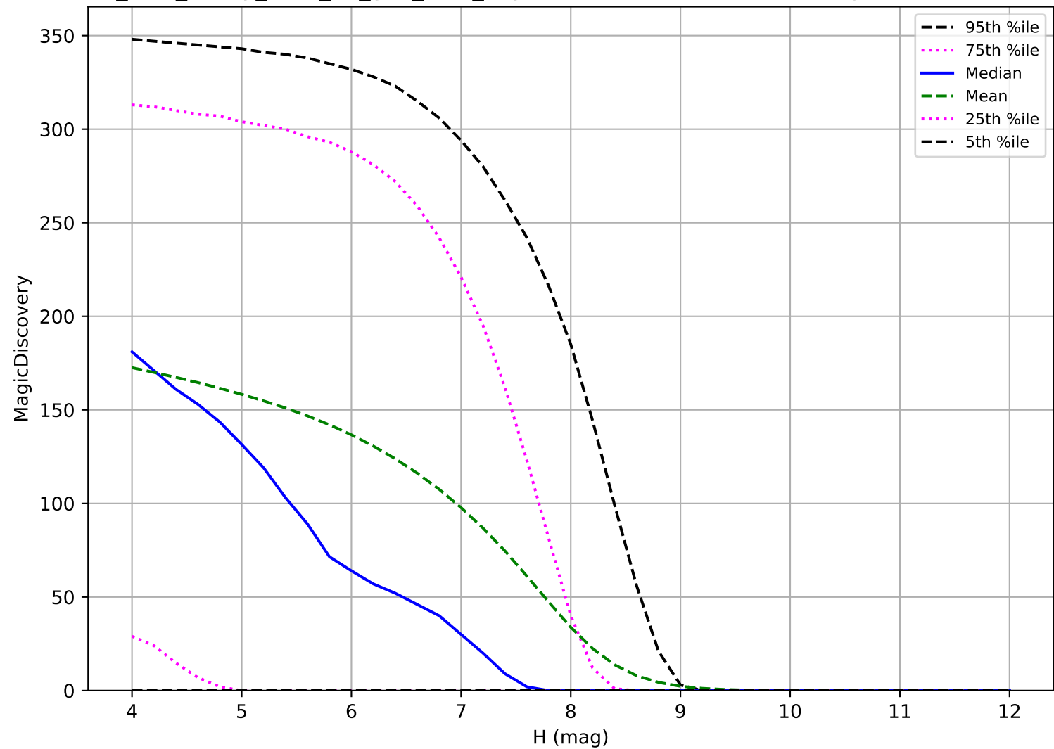
too_elab_heavy_r128_d2_griz_v3.4_10yrs: TNO 6 detections in 60 nights detection loss
