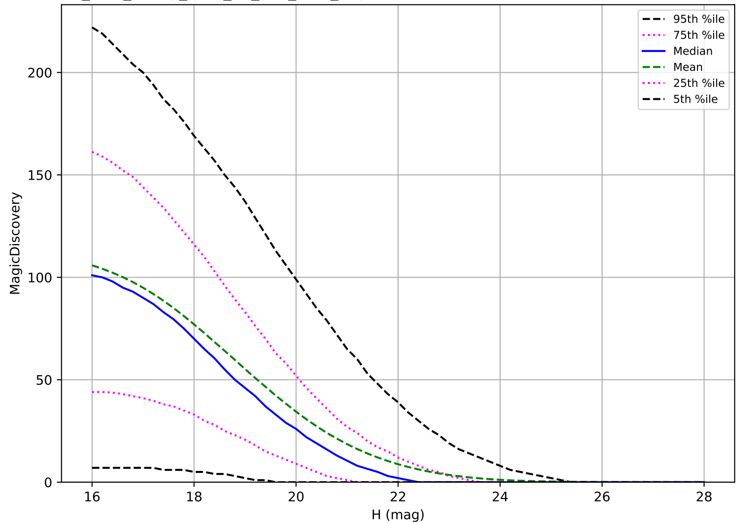
too_elab_heavy_r128_d2_griz_v3.4_10yrs: PHA 6 detections in 60 nights detection loss
