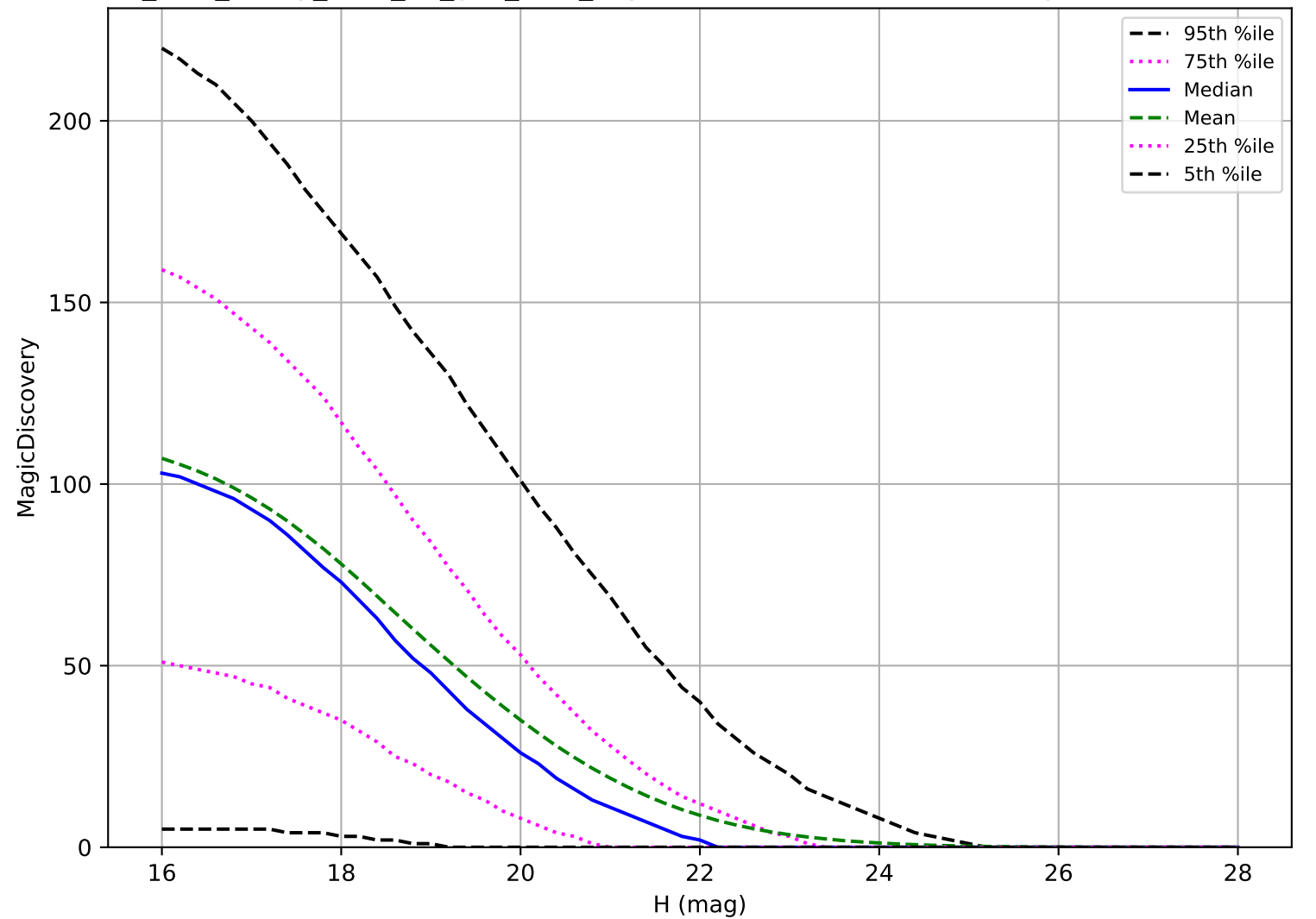
too_elab_heavy_r128_d2_griz_v3.4_10yrs: NEO 6 detections in 60 nights detection loss
