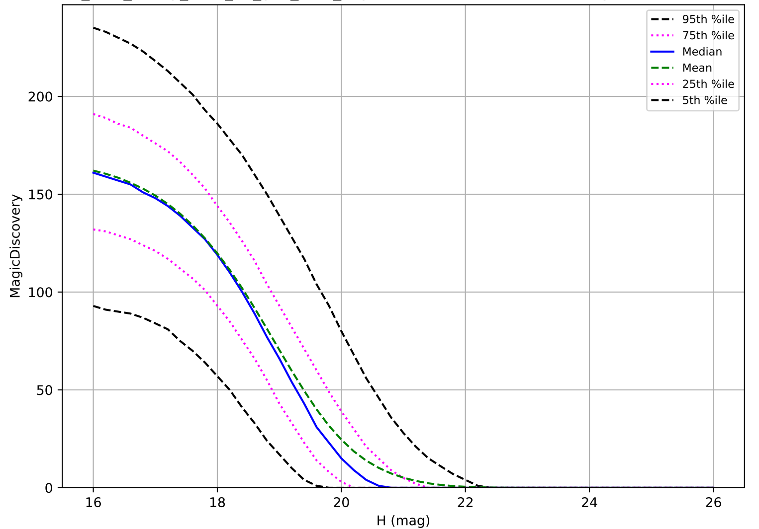
too_elab_heavy_r128_d2_griz_v3.4_10yrs: MBA 6 detections in 60 nights detection loss
