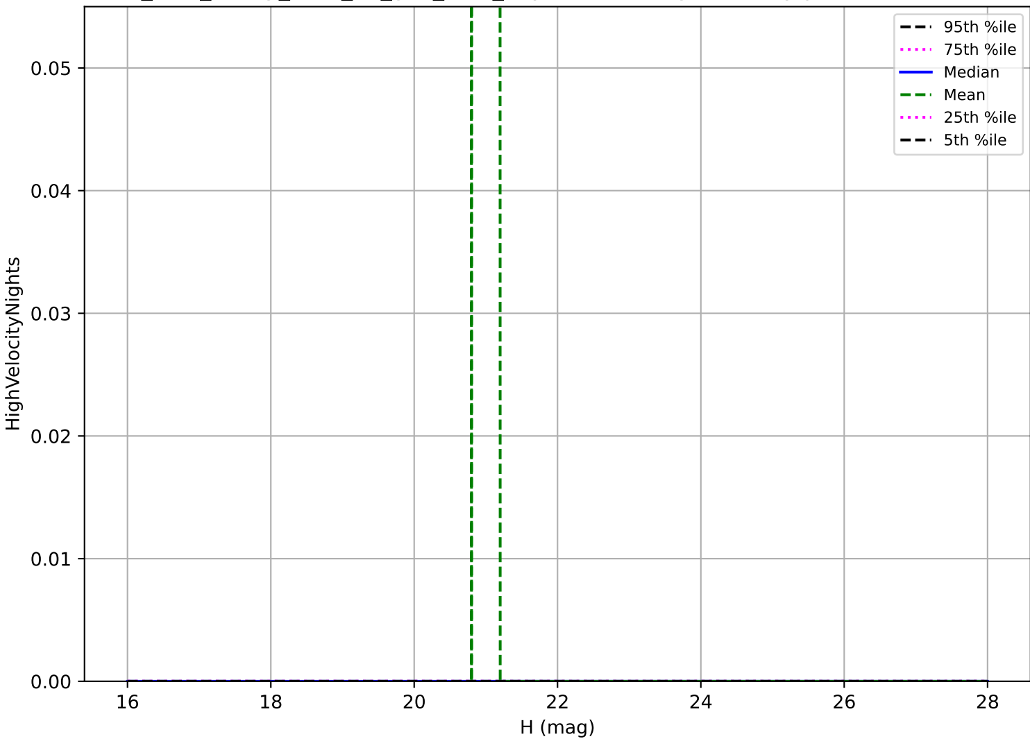
too_elab_heavy_r128_d2_griz_v3.4_10yrs: Vatira High velocity pair detection loss
