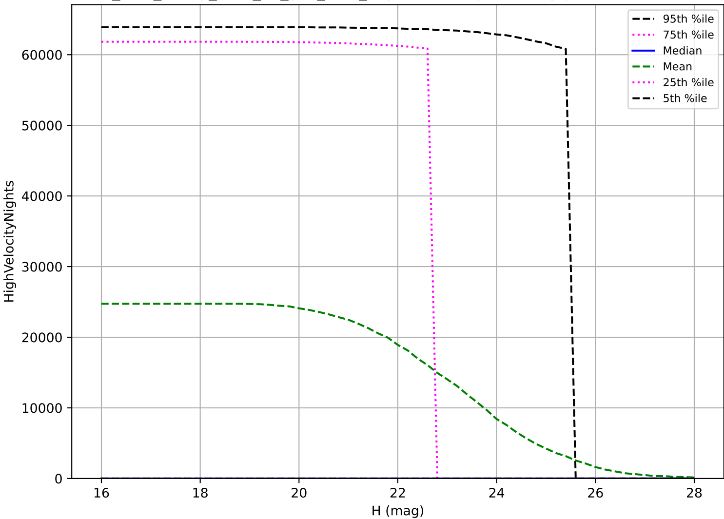
too_elab_heavy_r128_d2_griz_v3.4_10yrs: PHA High velocity pair detection loss
