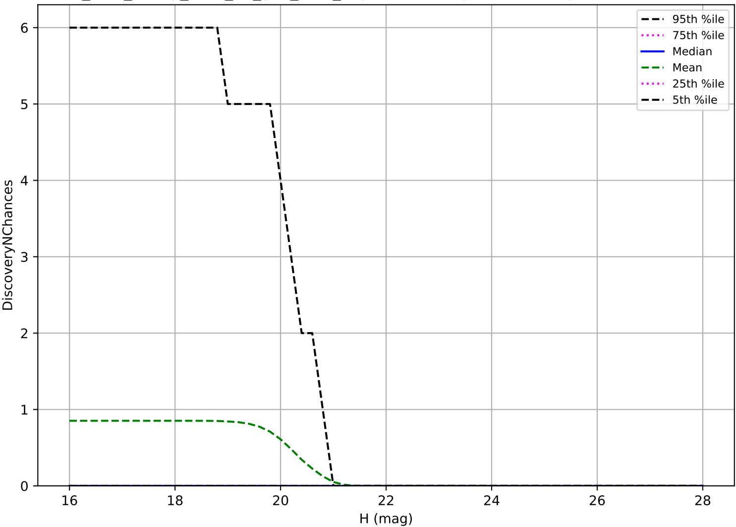
too_elab_heavy_r128_d2_griz_v3.4_10yrs: Vatira 3 pairs in 15 nights detection loss
