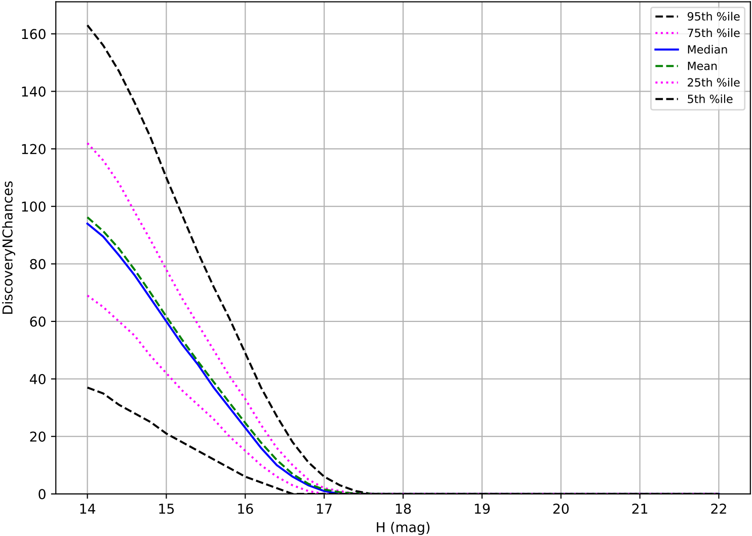
too_elab_heavy_r128_d2_griz_v3.4_10yrs: Trojan 3 pairs in 15 nights detection loss
