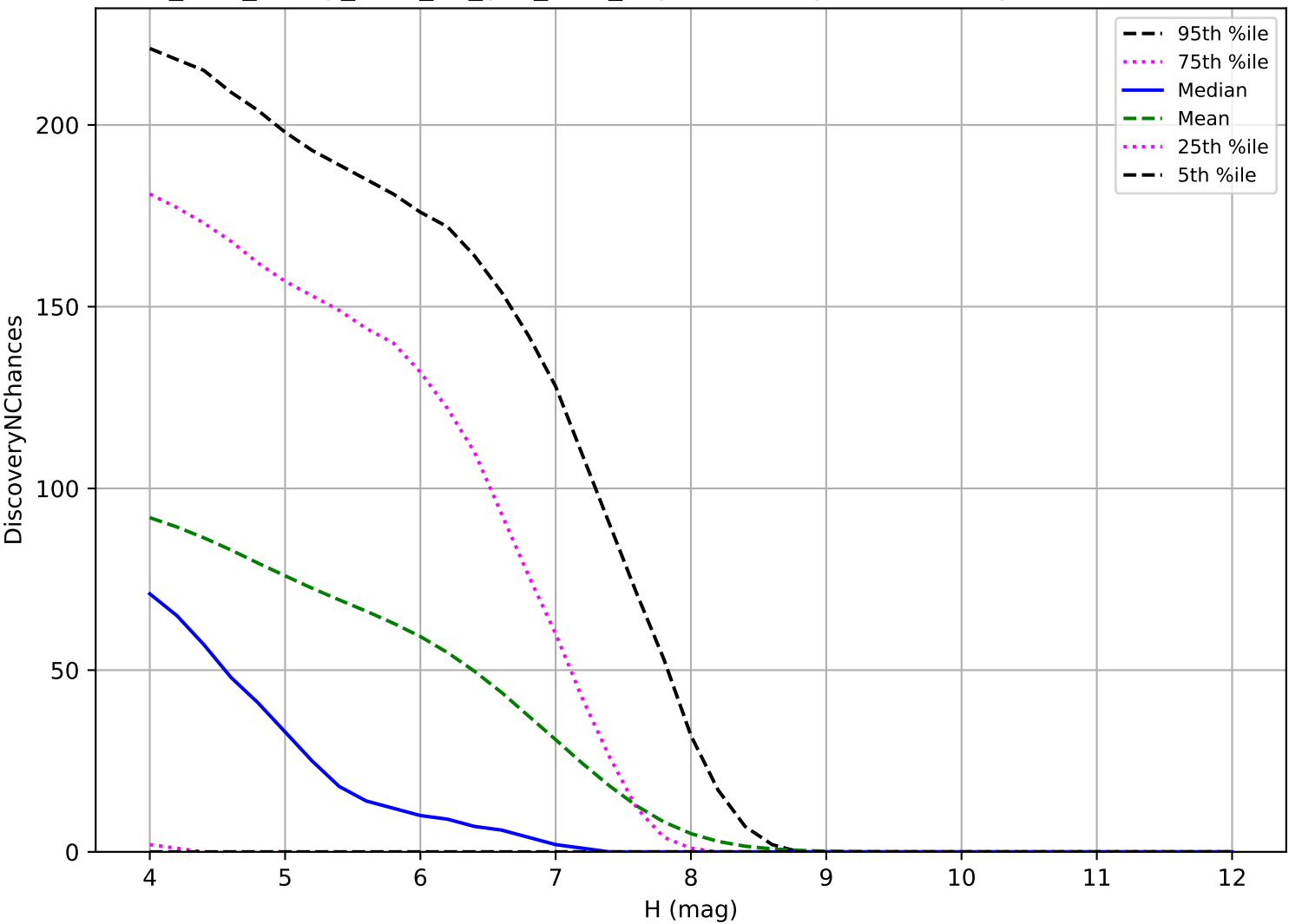
too_elab_heavy_r128_d2_griz_v3.4_10yrs: TNO 3 pairs in 15 nights detection loss
