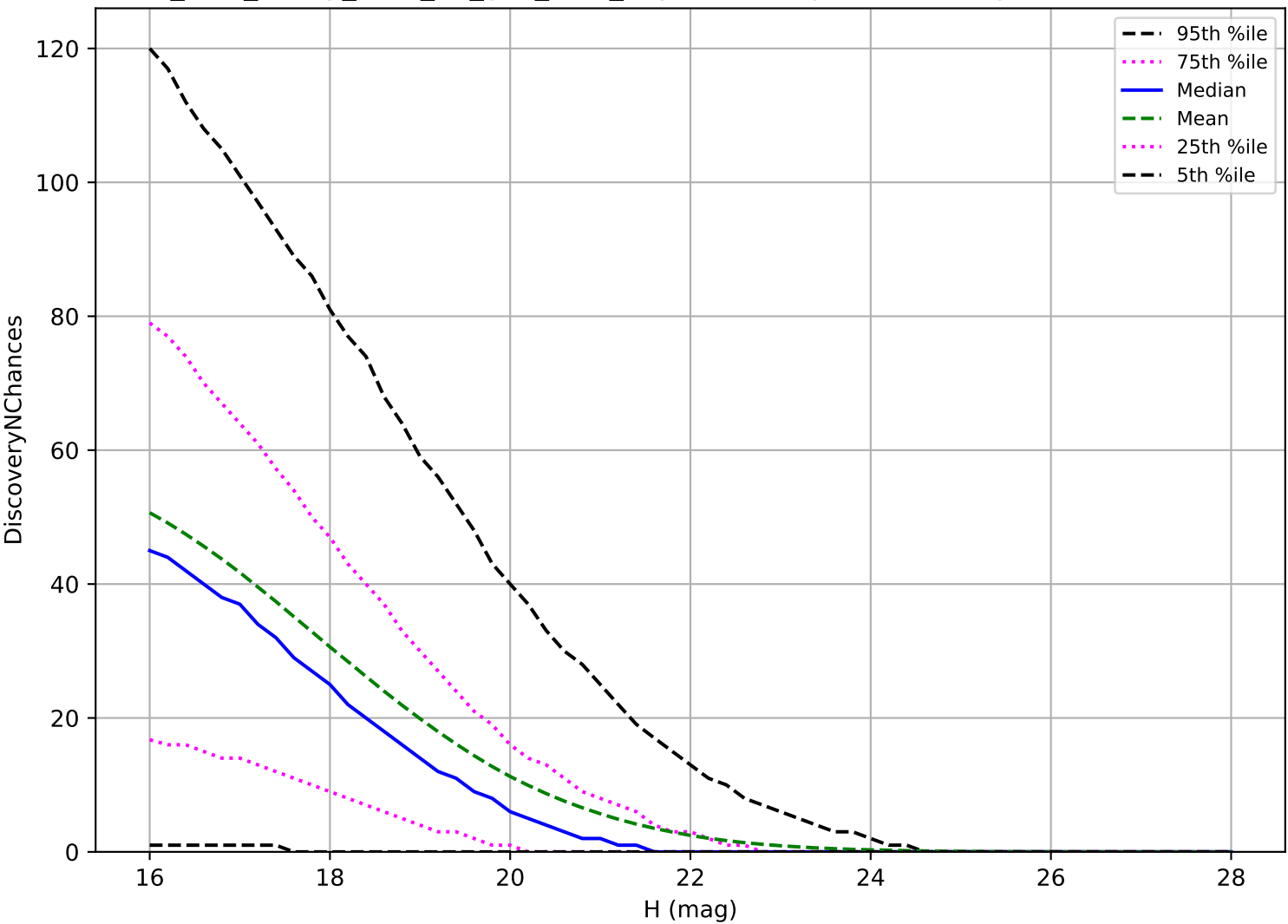
too_elab_heavy_r128_d2_griz_v3.4_10yrs: PHA 3 pairs in 15 nights detection loss
