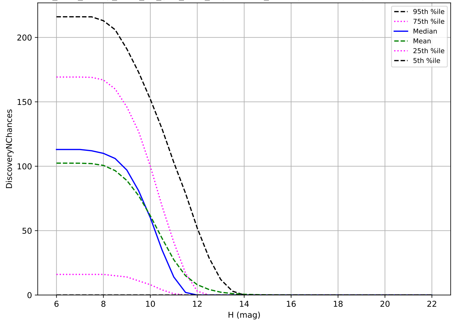
too_elab_heavy_r128_d2_griz_v3.4_10yrs: OCC_r20 3 pairs in 15 nights detection loss
